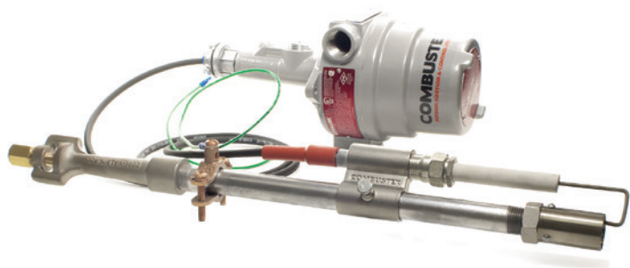
Ignition System with Pilot Tip and Flame Sensor
